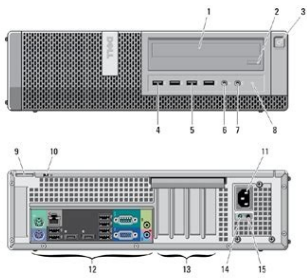
Figure 2. Front and Back View Of Desktop
